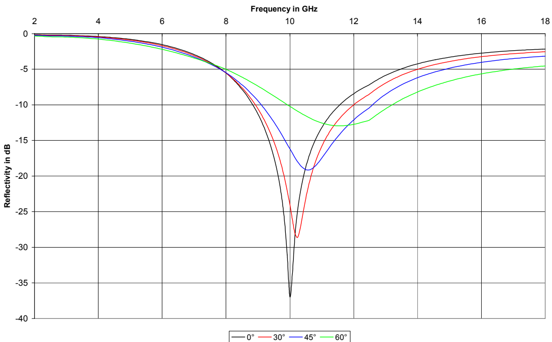
Typical reflectivity at various angles of incidence ECCOSORB DSF-U-10 Parallel polarization
